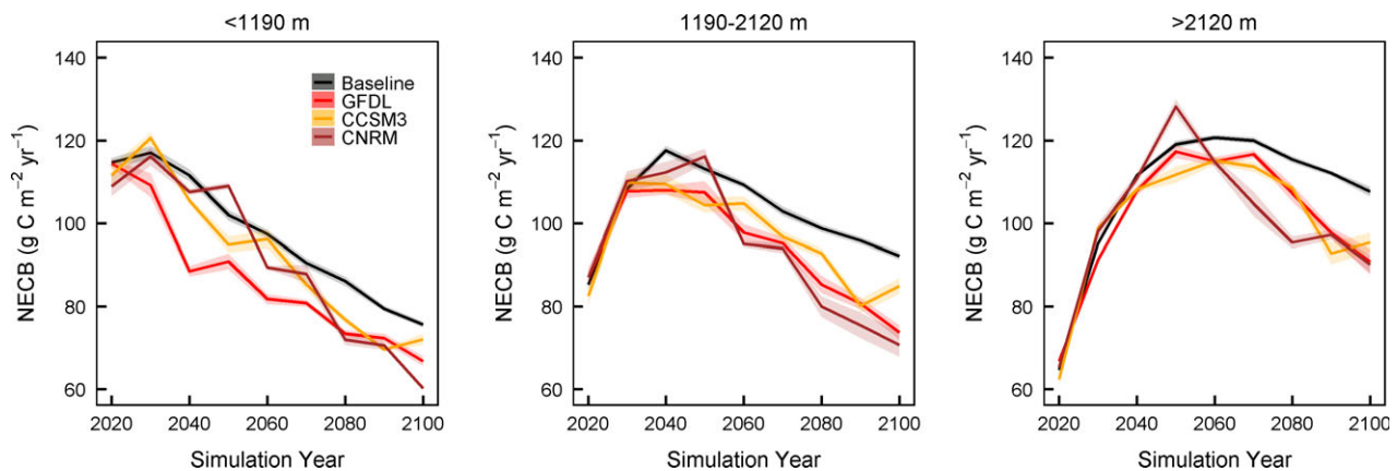
Fig. 4 Mean and standard error of landscape net ecosystem C balance (NECB) in each elevation band for baseline climate and wildfire and projected climate and wildfire under each climate model over the simulation period. Projected values are from five replicate simulations for each climate model. Baseline values are from three climate models and five replicate simulations.
