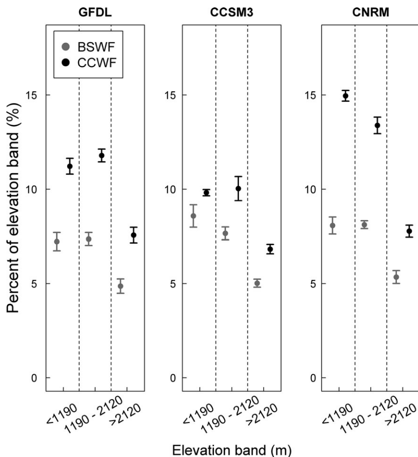
Fig. 5 Percentage of land area in each elevation band that is a C source by late century for each climate model under baseline climate and wildfire (BSWF) and projected climate and wildfire (CCWF). Values are mean and standard error for five replicate simulations for each climate model.
