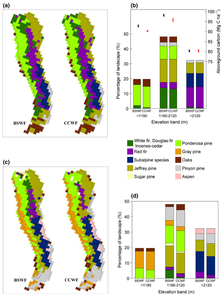
Fig. 2 The spatial distribution of dominant tree species by total biomass and species recruitment by largest number of new cohorts within each 12-km grid cell simulated under baseline climate and wildfire (BSWF) and projected climate and wildfire (CCWF). (a) Pixel values mapped at each grid cell are species with the highest biomass across five replicate runs and three climate models by late century (2100). (b) The hybrid bar plot shows the percentage of the landscape occupied by the species classes mapped in panel a within each elevation band under BSWF and CCWF. Mean and standard error of aboveground C by elevation band are presented using the right y -axis. Values are based on the mean across five replicate runs of the three climate models. (c) Pixel values mapped at each grid cell are the species with the largest number of new cohorts over the course of simulation across five replicate runs and three climate models. (d) The bar plot shows the percentage of the landscape occupied by the species classes mapped in panel c within each elevation band under BSWF and CCWF.
