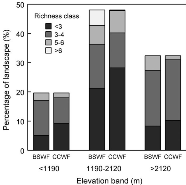
Fig. 3 The proportion of the landscape occupied by tree species richness class by elevation band under baseline climate and wildfire (BSWF) and projected climate and wildfire (CCWF). Values are based on the most frequent richness class within the 12-km grid cells across three climate models and five replicate runs by late century (2100).
