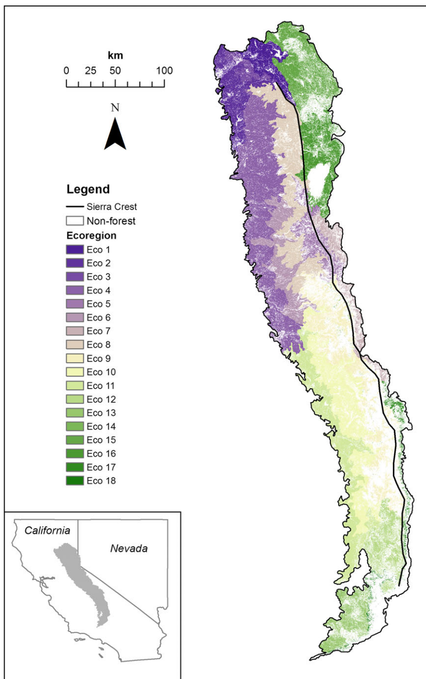
Fig. 1 Map of study area, the Sierra Nevada Mountains, CA, and NV, USA. Colored background shows the eighteen ecoregions used in LANDIS-II simulations. The black line shows the approximate location of the Sierra Nevada crest, differentiating the east and west slopes.
